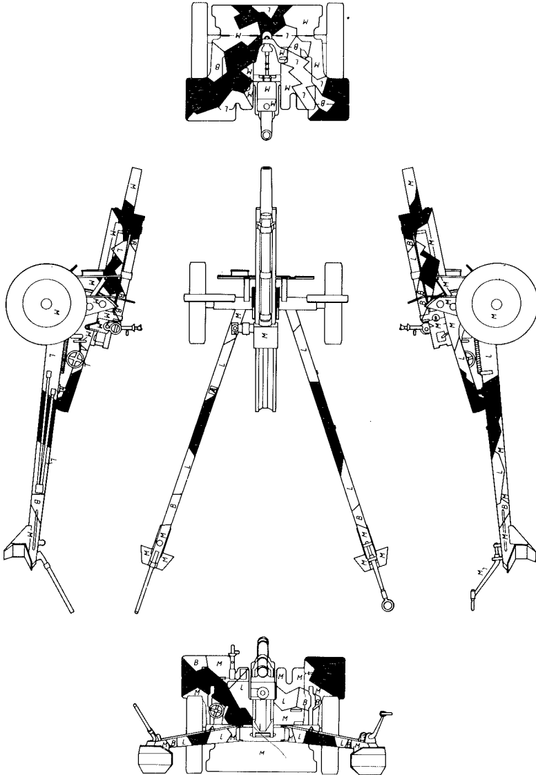
105 mm HAUBITS M 101
